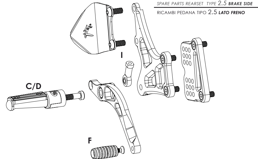
SPARE PARTS REARSET TYPE 2.5 BRAKE SIDE
